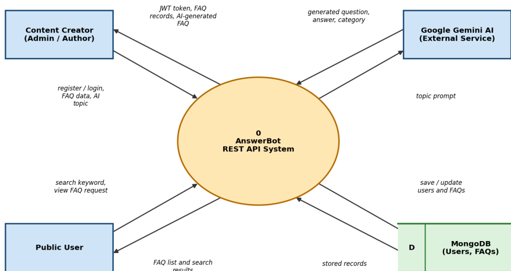
AnswerBot - Data Flow Diagram (Level 0 / Context Diagram)
